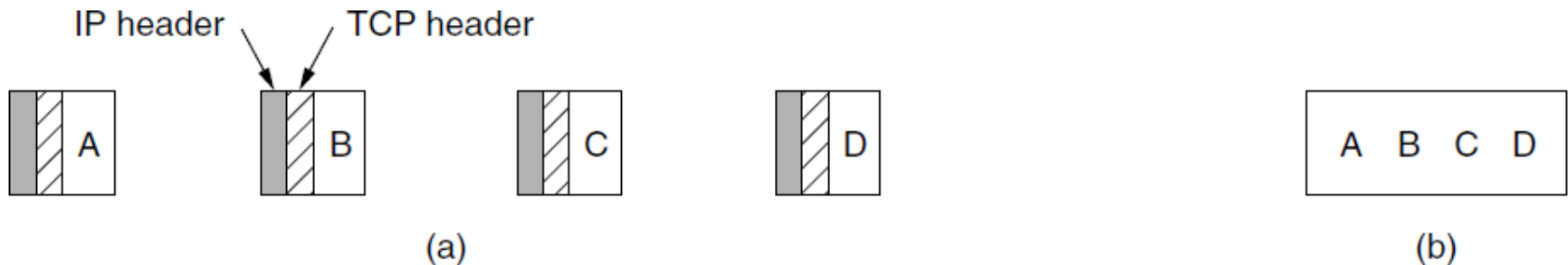
Figure 6-35. (a) Four 512-byte segments sent as separate IP datagrams. (b) The 2048 bytes of data delivered to the application in a single READ call.
